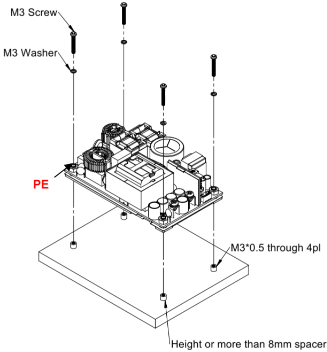
CFM500MXXX Installation Diagram
