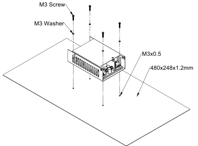
CFM500MXXXC installation diagram
