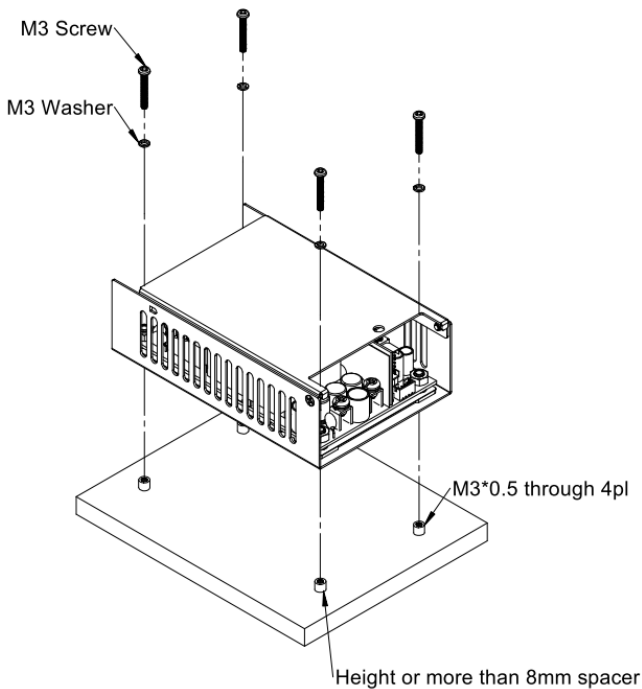
CFM500MXXXC Installation Diagram
